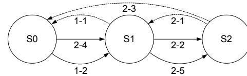
Figure 6. Re-dissemination w/ LGT & LRT
