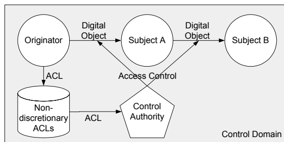
Figure 1. Traditional ORCON solutions
