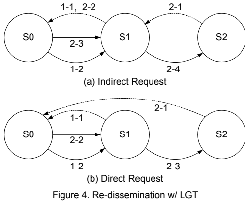
Figure 4. Re-dissemination w/ LGT
