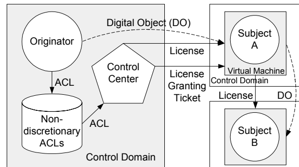
Figure 2. An example of ORCON w/ UCON
