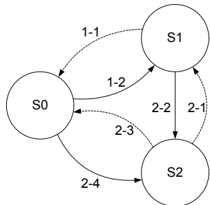
Figure 5. Re-dissemination w/ LRT
