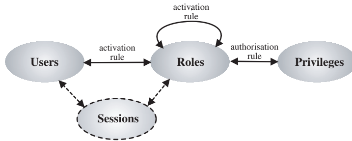
Figure 1. The basic Role-Based Access Control components.
