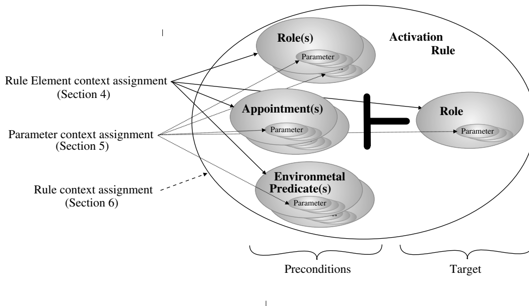
Figure 5. Role activation rule components that can be assigned a context.
