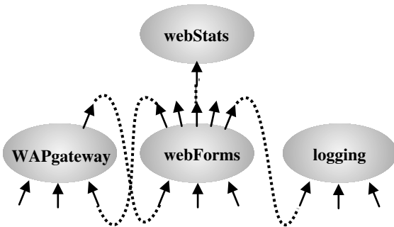
Figure 4. Example information flow among contexts.
